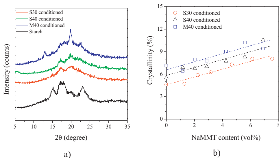
Fig. 2. Crystalline structure of TPS/NaMMT nanocomposites: (a) X-ray patterns of starch and TPS samples prepared by different methods; (b) Effect of clay content on the crystallinity of TPS nanocomposites.
