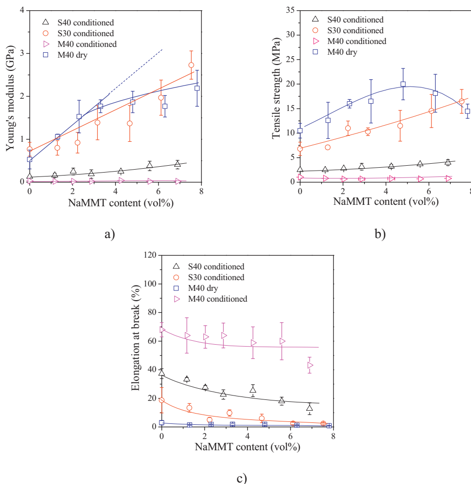
Fig. 7. Mechanical properties: effect of NaMMT content on the stiffness (a), strength (b) and elongation-at-break (c) of TPS/NaMMT nanocomposites
