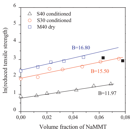
Fig. 8. Tensile strength of TPS/NaMMT nanocomposites plotted against filler content in the linear representation of Eq. (1).
