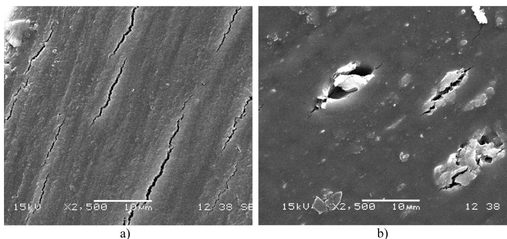
Fig. 5. Scanning electron micrographs recorded on the cryo-cut surfaces of S40-10 (a) and M40-10 (b) TPS/NaMMT nanocomposites.
