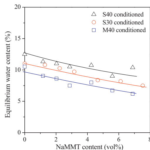
Fig. 6. Effect of filler and glycerol content as well as preparation technique on the equilibrium water content of TPS nanocomposites.
