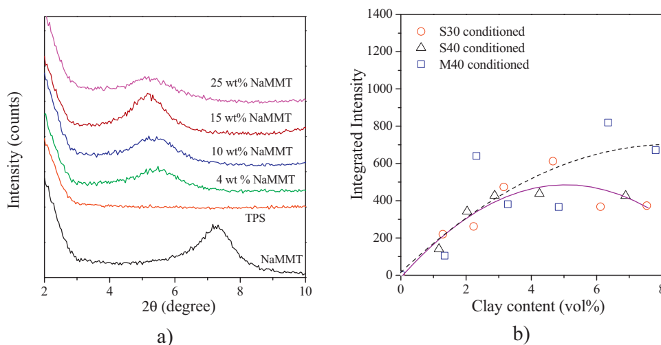
Fig. 3. X-ray results: (a) X-ray spectra of NaMMT, TPS and S30 nanocomposites; (b) Integrated intensity of the clay reflection plotted against clay content.
