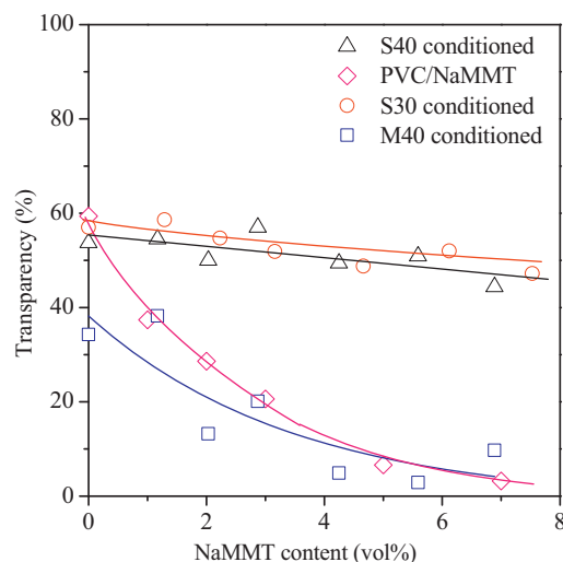
Fig. 4. Effect of clay content on the transparency of different TPS/clay and PVC/clay composites.
